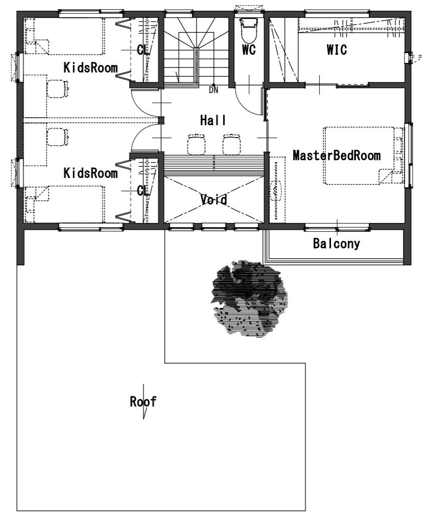
2F PLAN
