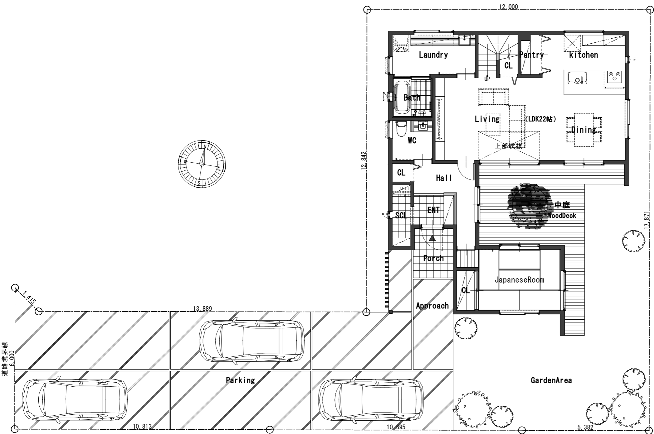
1F PLAN
